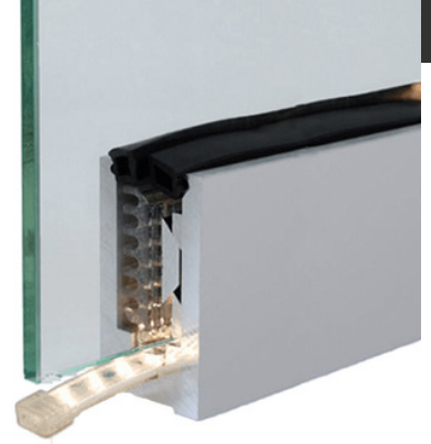
U channel
